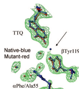
FIGURE 4. Active-site structures of MADH (blue) and \alpha 55A MADH (red). The structures of the ternary protein complexes with native (PDB, 2MTA) and \alpha 55A MADH (PDB, 1GM2) 22 are superimposed with the electron density for \alpha 55A MADH included. The single water present in the native active site and absent in the mutant is indicated by the arrow.
